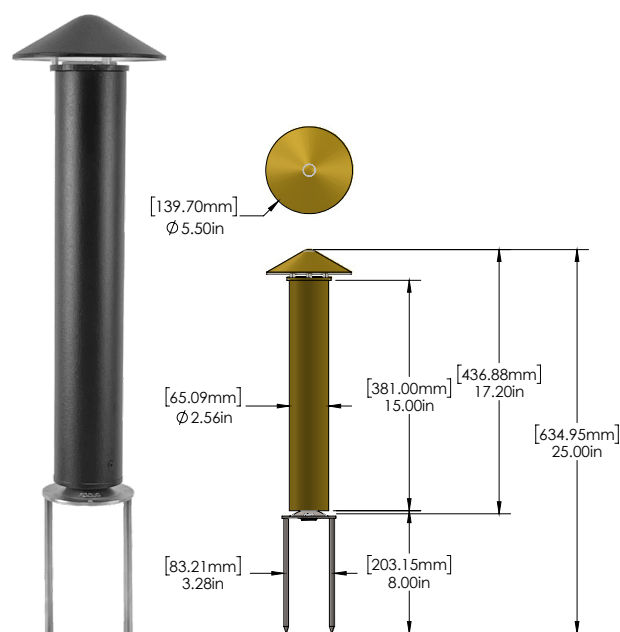
AL17SM2PL116BLT 12V AREA LIGHT WITH 2 PRONG MOUNTING STAKE
