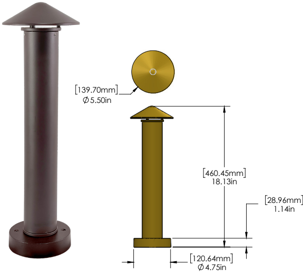
AL17SMDM2PL126BRSDZ 12V AREA LIGHT WITH 4.75" ROUND CANOPY DECK MOUNT Post Size: 15.00in x 2.00in dia. Height Options: 18.00in. (Standard) Hat: AL17SM Hat Options: See page 6 for more options Mounting: FA24LGCST 4.75" dia. Round Canopy Voltage Option: 120 Volt (See page 7)
