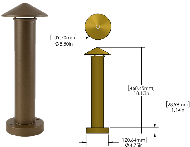
AL17SMDM2PL126BRT 12V AREA LIGHT WITH 4.75" ROUND CANOPY DECK MOUNT (DM)
