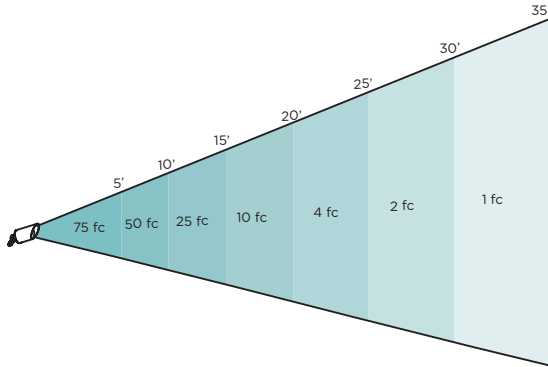
LRDM15 40°
