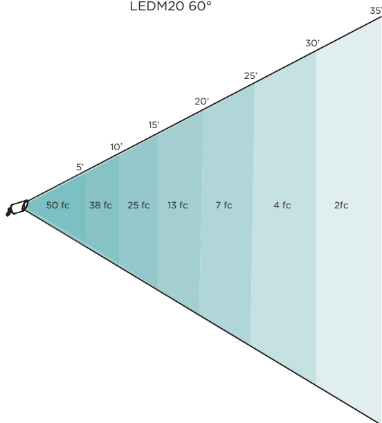
LED M20 60°
