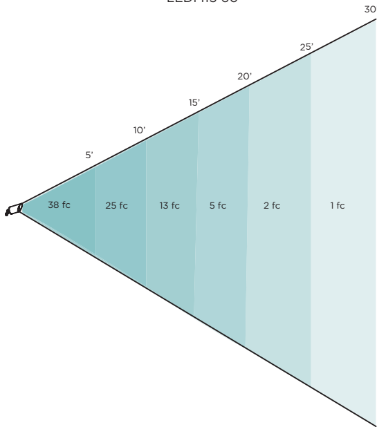
LED M15 60°
