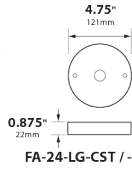
FA-24-LG-CST / -BRS FA-24-LG-SPUN / -BRS (12-277v)
