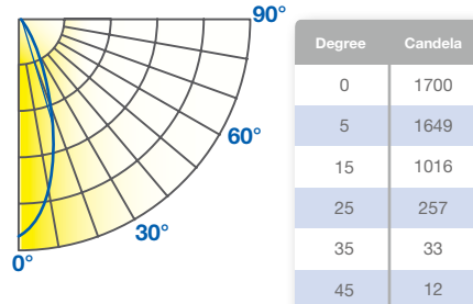
FL-LED-MR16GC-85D-30-35
