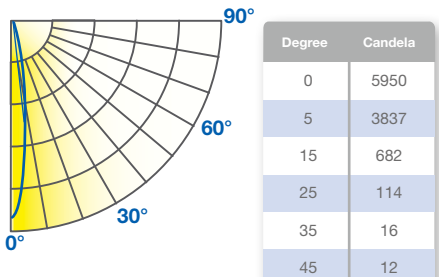
FL-LED-MR16GC-85D-30-15
