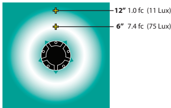
SL-20-SMM Light Distribution
