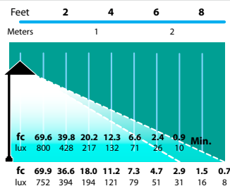
PL-14 Half Spread Photometrics 18 ft. (5.5m) diameter
