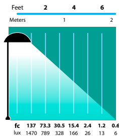
PL-11 Half Spread Photometrics 14 ft. (4.2m) diameter
