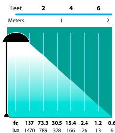
PL-11 Half Spread Photometrics 14 ft. (4.2m) diameter
