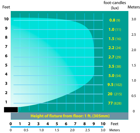
FFL-13-CST Half Spread Photometrics
