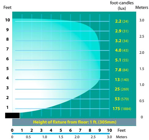
FFL-26-CST Half Spread Photometrics
