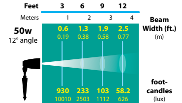
FL-10-EXT-FG FL-10-EXT-ULTRA
