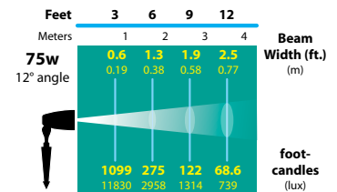
FL-20-EYF-FG
