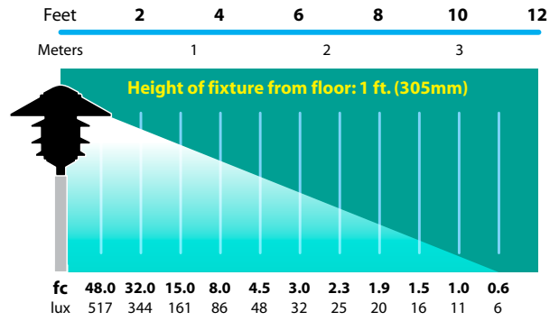
IAL-04-10 Half Spread Photometrics (40w) 22 ft. (6.7m) diameter
