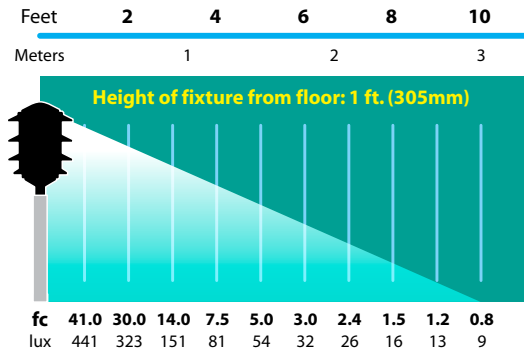
IAL-04 Half Spread Photometrics (40w) 18 ft. (5.5m) diameter
