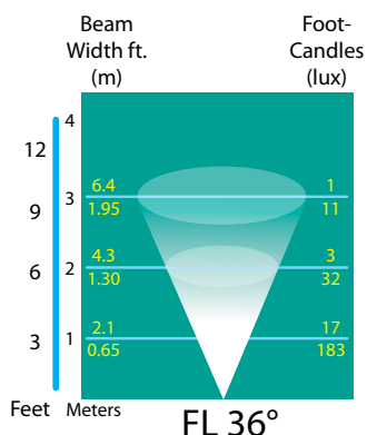
FL-LED-MR16SS5W36
