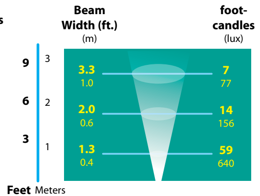
15° MR11 LED
