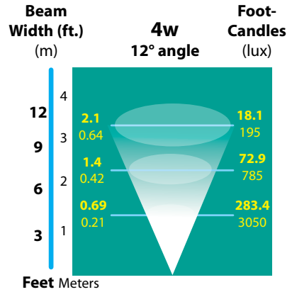
12° MR16 LED
