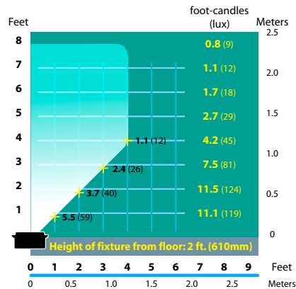
SL-31 Half Spread Photometrics
