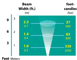
15° PAR20 ARROW LED
