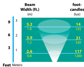
40° PAR20 ARROW LED
