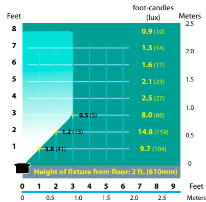
SL-17 Half Spread Photometrics
