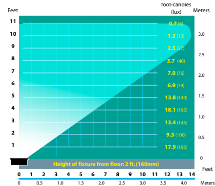
SL-08-T10 Half Spread Photometrics
