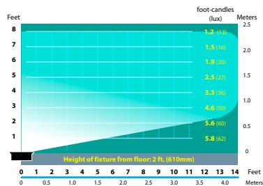
SL-08-AL-FL-5 Half Spread Photometrics (5w)
