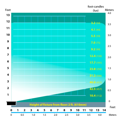
SL-08-FL-9 Half Spread Photometrics (9w)
