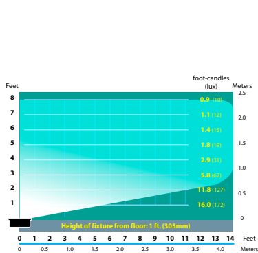
SL-08-FL-5 Half Spread Photometrics (5w)
