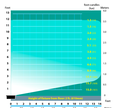
SL-08-AL-FL-9 Half Spread Photometrics (9w)
