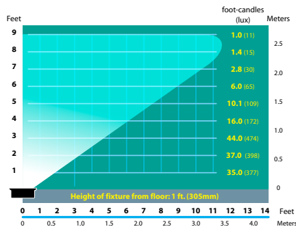
SL-08-T10 Half Spread Photometrics
