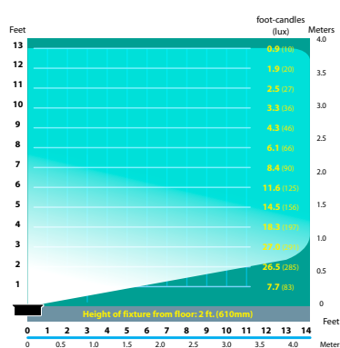
SL-08-FL-7 Half Spread Photometrics (7w)
