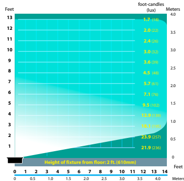
SL-08-AL-FL-7 Half Spread Photometrics (7w)
