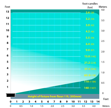
SL-08-FL-9 Half Spread Photometrics (9w)
