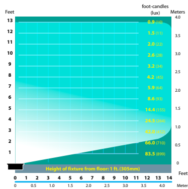
SL-08-FL-7 Half Spread Photometrics (7w)
