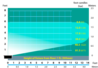
SL-08-AL-FL-7 Half Spread Photometrics (7w)
