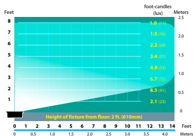
SL-08-FL-5 Half Spread Photometrics (5w)
