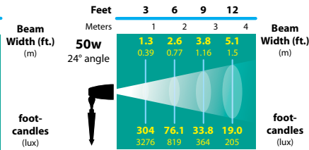
FL-10-EXZ-ULTRA
