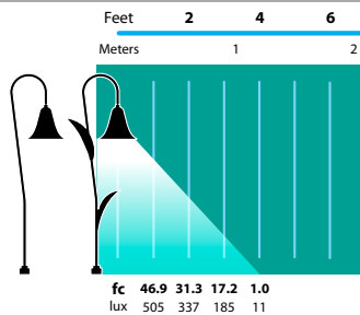
PL-02, PL-02-LVS Half Spread Photometrics
