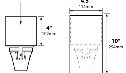
PGL-05 SLEEVE (Supplied)
