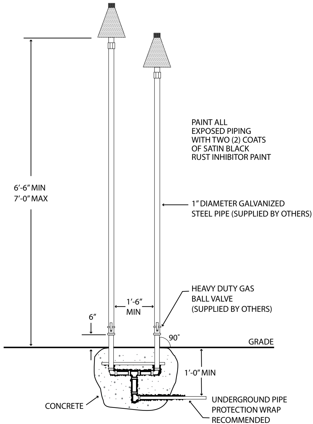
Installation Diagram #1
