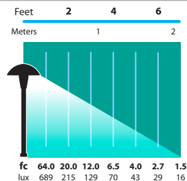
AL-11 Half Spread Photometrics 14 ft. (4.3m) diameter
