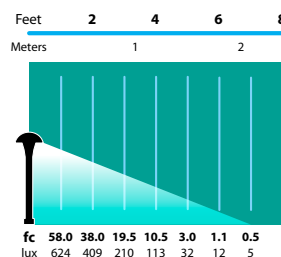
AL-06-SM Half Spread Photometrics 14 ft. (4.3m) diameter
