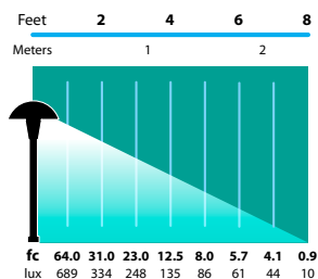
AL-06 Half Spread Photometrics 16 ft. (4.9m) diameter
