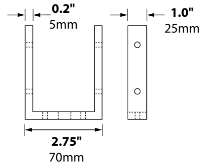
U-Bracket Detail
