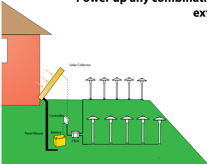
FOCUS 100w 12v DC LED SOLAR SYSTEM ON GROUND MOUNT
