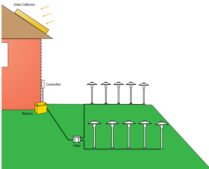
FOCUS 100w 12v DC LED SOLAR SYSTEM MOUNTED ON ROOFTOP
