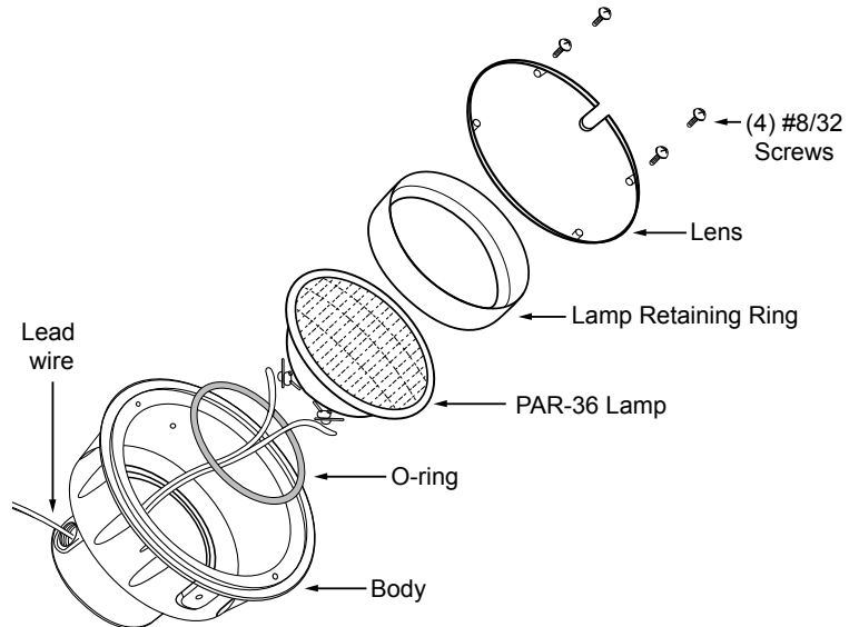
SL-11 (exploded view)
