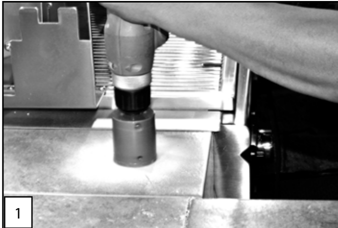
(1) Drill 2" hole through surface. A wet drill is recommended for hardscape installs. CAUTION: Make sure area underneath is clear of wire, conduit, gas lines, etc.
