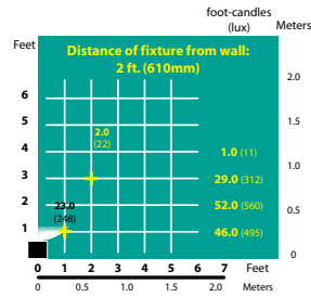
DL-04-HE Half Spread Photometrics
