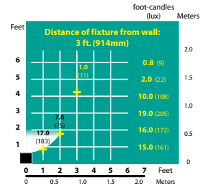
DL-04-HE Half Spread Photometrics
