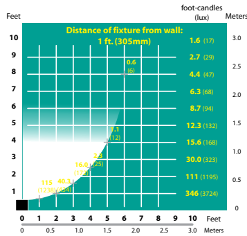
DL-04 Half Spread Photometrics
