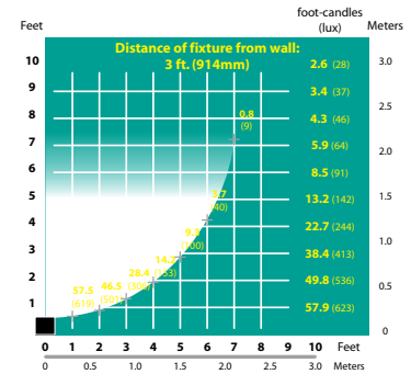
DL-04 Half Spread Photometrics
