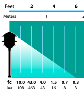
AL-03-3T Half Spread Photometrics 12 ft. (3.7m) diameter
