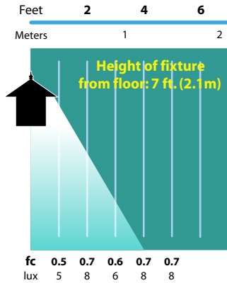
SL-12 Half Spread Photometrics 8 ft. (2.4m) diameter
