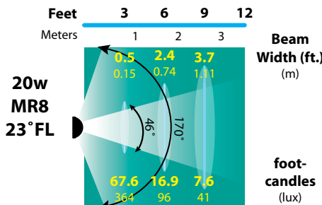
SL-07 Half Spread Photometrics
