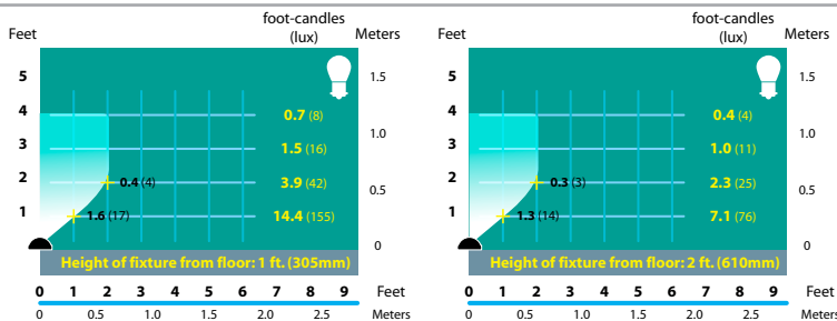
SL-07 Half Spread Photometrics
